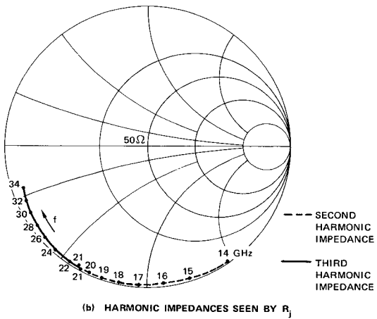
(b) HARMONIC IMPEDANCES SEEN BY R_1
