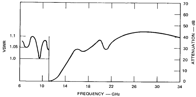
(a) VSWR AND ATTENUATION
